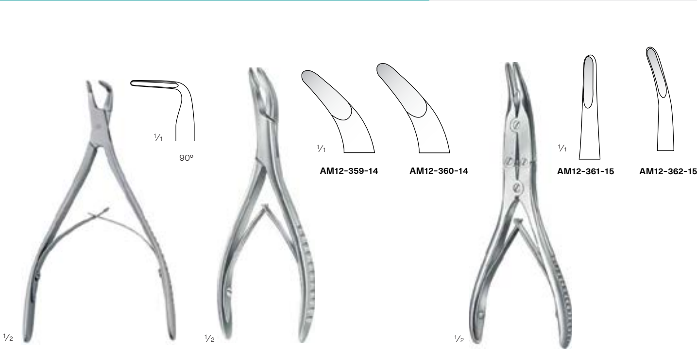
Luer AM12-359-14 - AM12-360-14 14,5 cm / 5 9/16"
