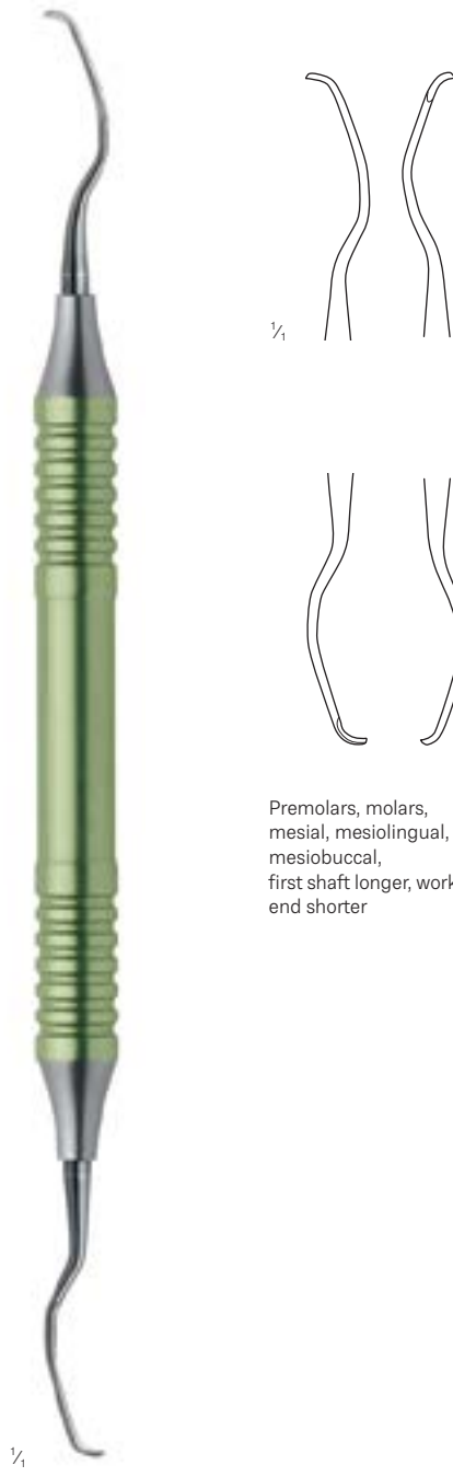
AM29-152-12 Ti Fig. 11/12 17,5 cm / 6 7/8" hollow handle, 10 mm
